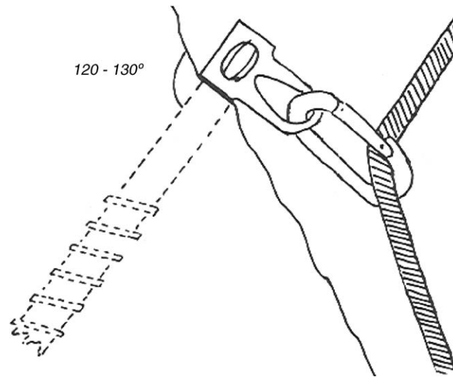
Fig. 1. The ice-screw's eyelet has to point in the direction where the strain will come (from "Skandinavisk Høyfjellsutstyr A/S katalog 1984–85" Printed by permission of T. Carlstrøm).
