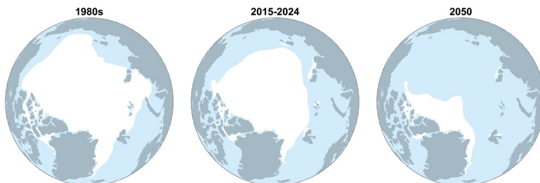
Figure 2: From a white to a blue Arctic Ocean. Arctic Ocean sea ice extent in September defined as regions with sea ice concentration of more than 15%, for a situation typical for the 1980s (5.5 million km 2 ), the last decade (3.3 million km 2 ), and for a practically sea ice-free Arctic Ocean (<1 million km 2 ), which is expected to occur before 2050. The sea ice lost since the 1980s is more than 5 times larger than the area of mainland Norway. An ice-free Arctic Ocean would mean that sea ice corresponding to an area about half the size of Europe is lost. Figure based on data from Jahn et al. (2024).
