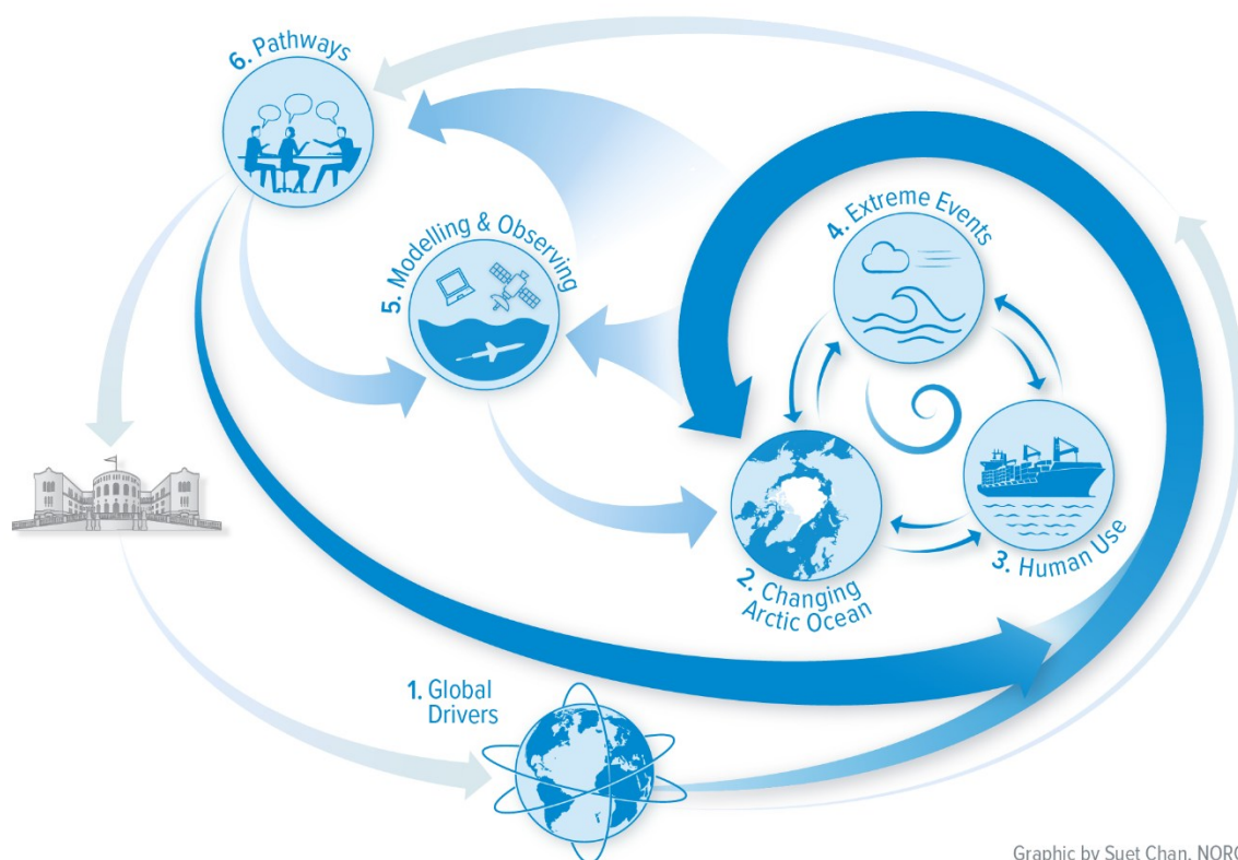
Figure 6: Structure of Polhavet / Arctic Ocean 2050. The Polhavet / Arctic Ocean 2050 programme is organized into six Research Themes (RTs) that collectively ensure a transdisciplinary approach. The first four RTs focus on closing key knowledge gaps on the region's environmental conditions and influences, marine life, human use, and governance. The fifth RT focuses on advancing technological solutions for better research and management, and the sixth will integrate the knowledge generated in close collaboration with stakeholders. © Suet Chan, NORCE
