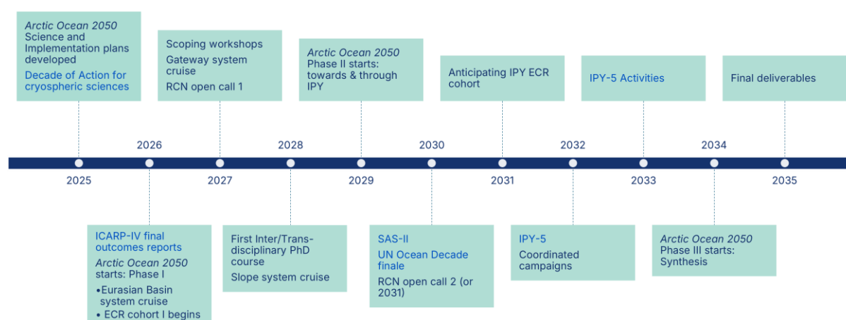
Figure 4: International Context. Polhavet / Arctic Ocean 2050 in the context of relevant Arctic-focused international processes.
