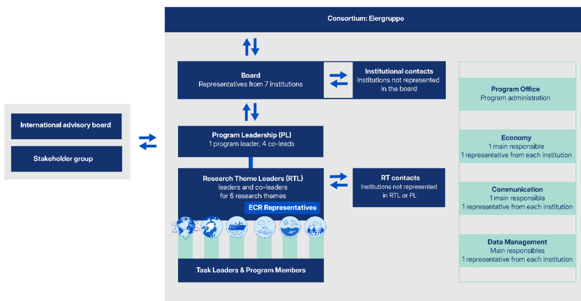
Figure 8: Organisation of Polhavet / Arctic Ocean 2050. Organigram representing the Board and institutional contacts, Programme Lead team, Research Theme leader group and members, as well as the International Advisory Board, Transdisciplinary actors (in formation), Data Management, Communication groups, Programme office and economic support. © Polhavet / Arctic Ocean 2050
