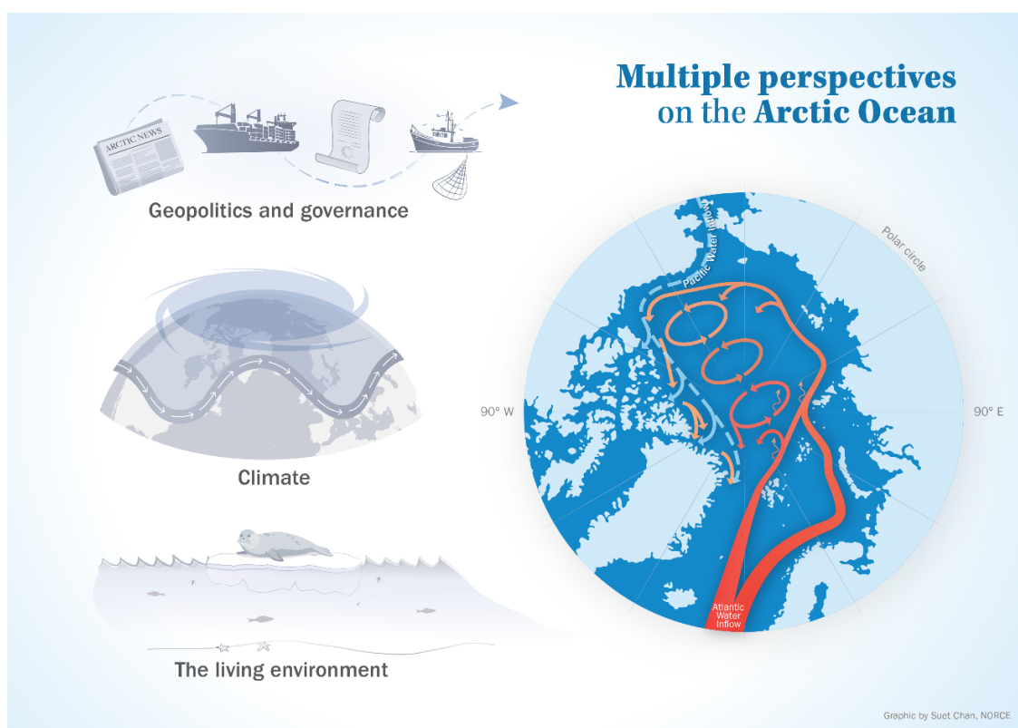
Figure 1: The multiple perspectives of Polhavet / Arctic Ocean 2050 . © Suet Chan, NORCE.
