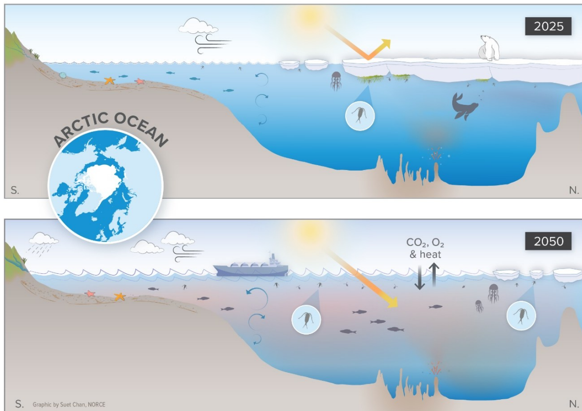
Figure 3: A changing Arctic Ocean. Idealized section across the Arctic Ocean from the shelf to the North Pole showing expected summer-time changes toward 2050, including a warmer, less ice-covered, and more productive ocean, with ecosystem components, including fish populations, and human activity moving northward (note that the schematics are not to scale). © Suet Chan, NORCE
